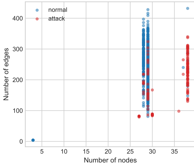
LID-DS (Bruteforce_CWE-307)
