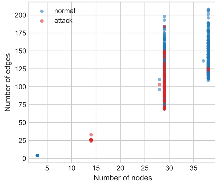
LID-DS (CVE-2014-0160)
